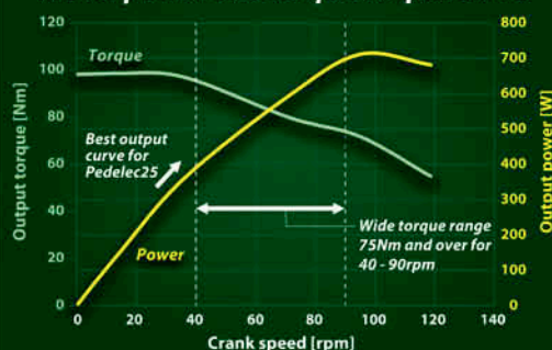
Motor power and torque output curve
