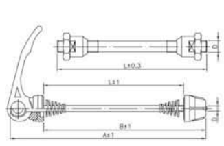
Model A101/ A102 Axle Length (L): 108/ 136 , 140 , 145 Material: Steel Weight:100g/ 400g
