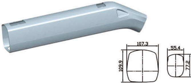
3 SUSPENSION MOTOR MOUNT: HSMM-242111
