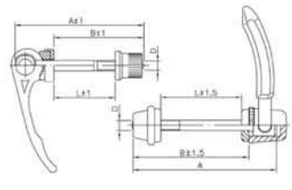
Model F90-AYAK / R90-AYAK -Tire Remover + QR Weight:64g/ 71g
