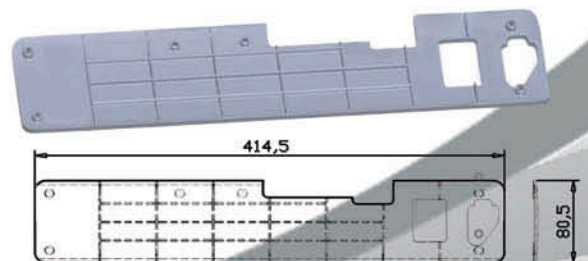
8 BATTERY COVER: HBC-41581
