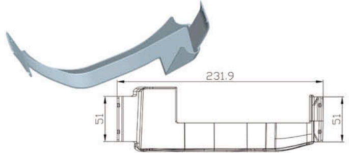
8 BATTERY COVER: HBC-41581
