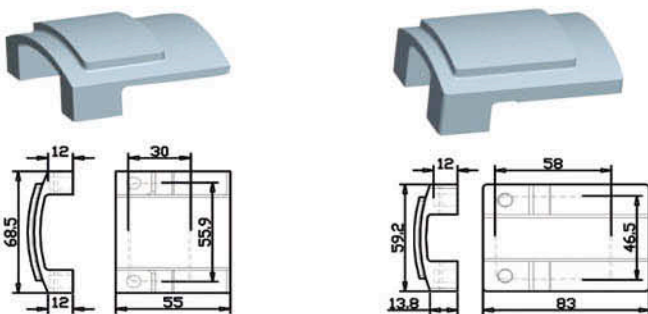
7 BATTERY MOUNT: HBM-6955/HBM-8359
