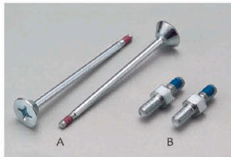
Model SGB-049 A: Hex Cross Flat Head, Size: M3 B: Special Bolt, Size: M5 Finish: UCP
