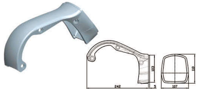
4 LADY MOTOR MOUNT: HLMM-185110
