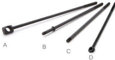
Model : SHL 04 Bolts for front and rear quick release axle Size : M5*100~300mm
