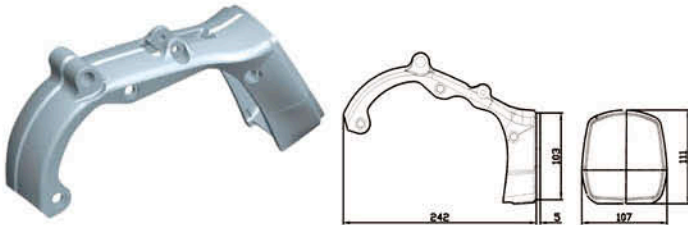
5 MOTOR COVER: HMC-23171
