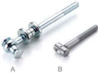
Model : SHL 03 For seat quick release A、B : M5/M6 length and color is optional
