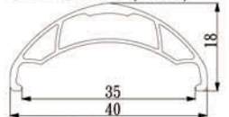
MB4.0 Sleeved joint Size:29"/27.5"(650B)
