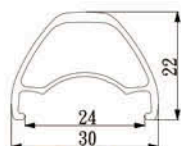
GTD30 Sleeved / Weld joint Size:29"/27.5"(650B)
