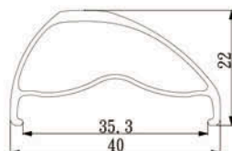
OCR4.0d Sleeved joint Size:29"/27.5"(650B)
