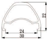
GTD30 Sleeved /Weld joint Size:29"/27.5"(650B)/24" for tubeless ready
