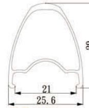
RD29 Sleeved joint Size:700C/650C
