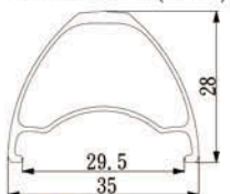
GTD35 Sleeved / Weld joint Size:29"/27.5"(650B)
