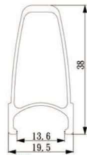
XF Weld joint Size:451/406
