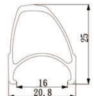
OCR25 - 16 Sleeved joint Size:451/406/355/349
