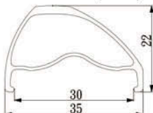
OCR3.5d Sleeved joint Size:29"/27.5"(650B)
