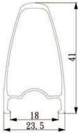
XRD Weld joint Size:700c for tubeless ready
