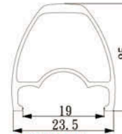
GTD25 Sleeved joint Size:700C/650C
