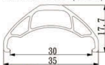
MB3.5 Sleeved joint Size:29"/27.5"(650B)
