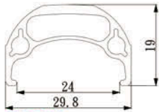
BM30 Pin joint Size:29"/27.5"(650B)/ 24"/20"
