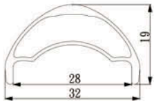
MB3.2h Sleeved joint Size:29"/27.5"(650B)
