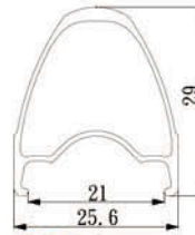
RV29 Sleeved joint Size:700C/650C
