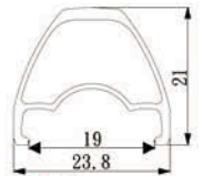
X35 Sleeved / Weld joint Size:700C /650B
