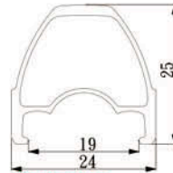
GTM25 Sleeved joint Size:700C/650C
