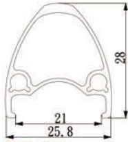
XD28 Pin joint Size:29"/27.5"(650B)/24" for tubeless ready
