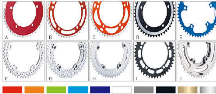
SS-8106 Chainring: 39, 42, 44, 46, 48, 50, 52T. Steel or alloy Crank: Forged 6061/T6 alloy Length: 165, 170, 175mm BCD: 130mm Chainline: 43mm Axle length: 103mm
